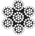
7 x 19 7 strands 19 wires/strand
