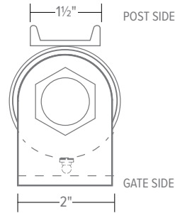
PART 2115P Flat to Gate, Round to Post Primed 1
