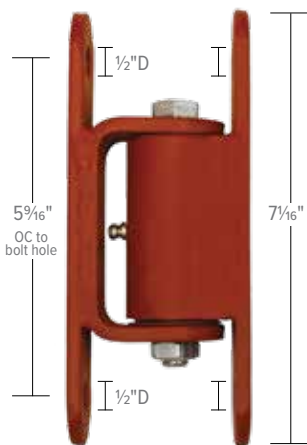
PART 2150P Bolt to Gate, Bolt to Post Primed 1 PART 2150Z Bolt to Gate, Bolt to Post Zinc 1 PART 2150B Bolt to Gate, Bolt to Post Black PC 1
