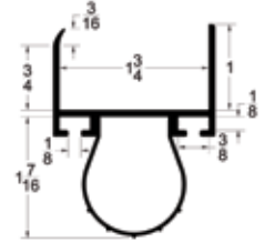
1 3/4" AR-175 ASTRAGAL
