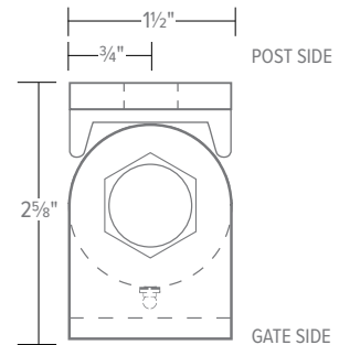
PART 2125P Flat to Gate, Bolt to Post Primed 1
