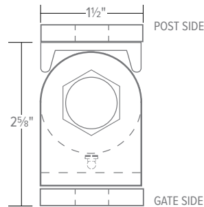
PART 2150P Bolt to Gate, Bolt to Post Primed 1 PART 2150Z Bolt to Gate, Bolt to Post Zinc 1 PART 2150B Bolt to Gate, Bolt to Post Black PC 1
