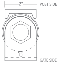
PART 2100P Flat Mount, Both Sides Primed 1 PART 2100U Flat Mount, Both Sides No Finish 1 PART 2100Z Flat Mount, Both Sides Zinc 1
